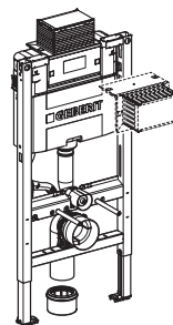
Duofix 98 Omega 111.030.00.2
