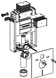
Combifix 98 Omega 110.010.00.1
