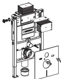
Duofix 90 Omega 111.016.00.2
