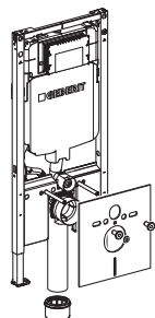
Duofix Sigma8 111.795.00.2
