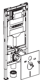
Duofix Sigma12 111.907.00.6 111.908.00.6 111.909.00.6
